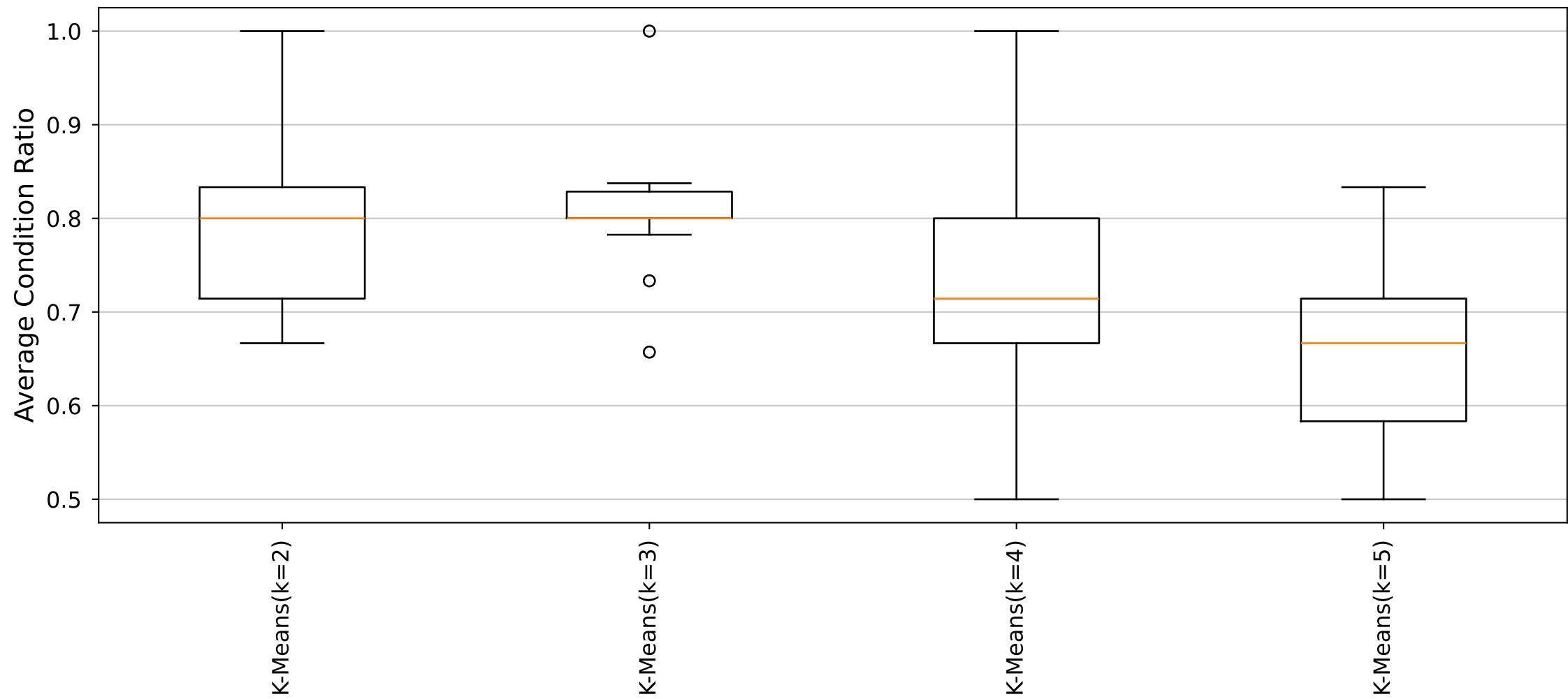
YARA Rules Average Condition Ratio Distribution (Cluster38_Size5 dataset)
